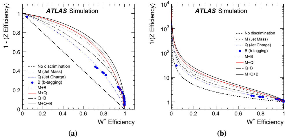
Fig. 8 The tradeoff between W^+ efficiency and a 1 - (Z \text{ efficiency}) or b 1/(Z \text{ efficiency}) on a a linear scale and b a logarithmic scale. Each curve is constructed by placing thresholds on the likelihood constructed
